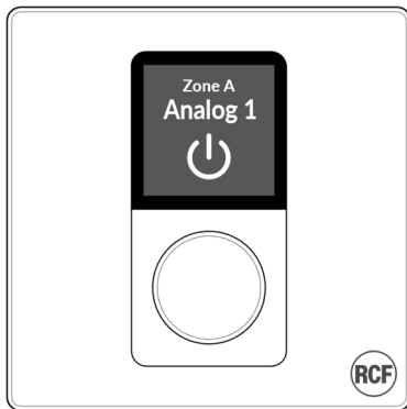
Main screen
