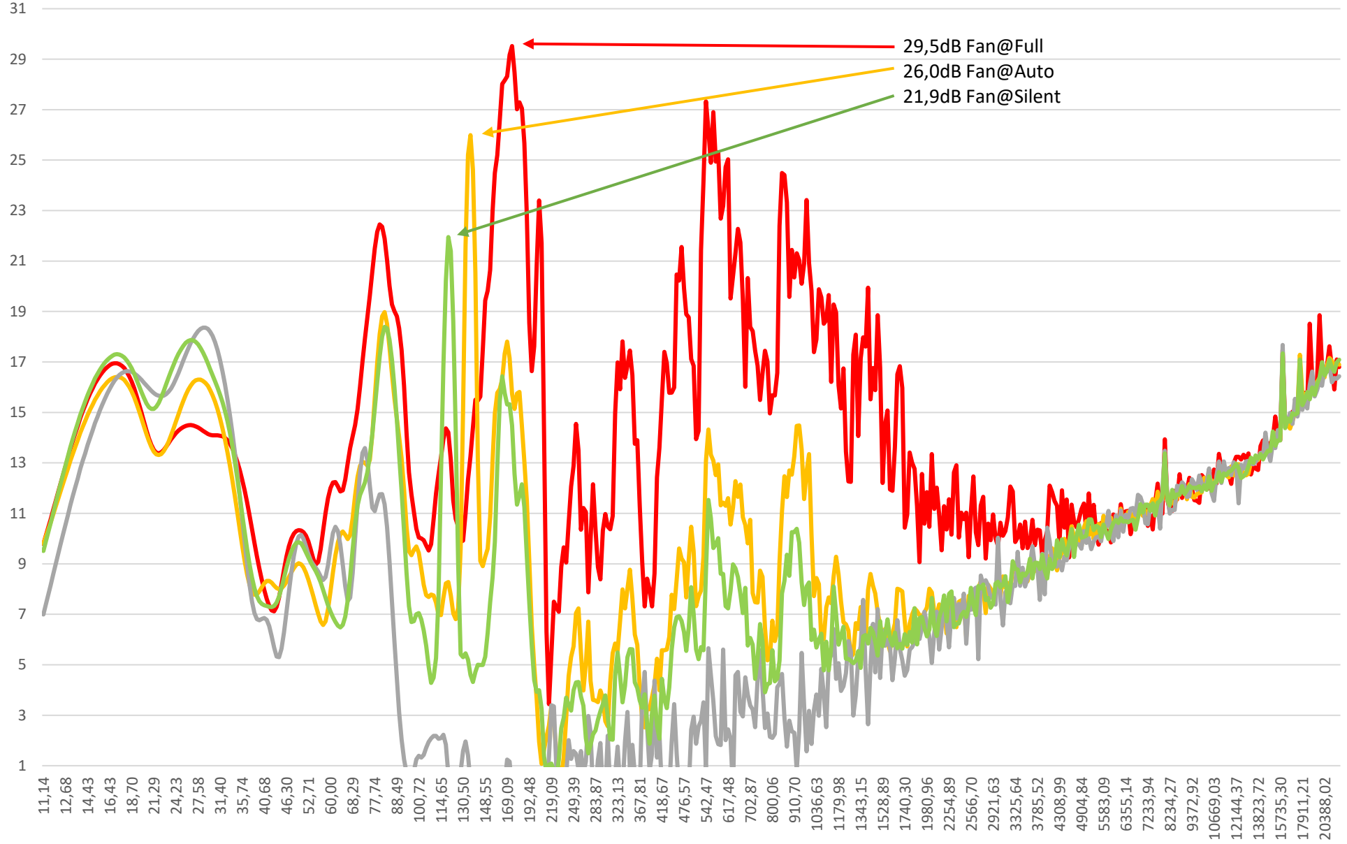
Infinity Signature TF-260C7 Noise Level measurement @ operation temperature 50-55 degrees
