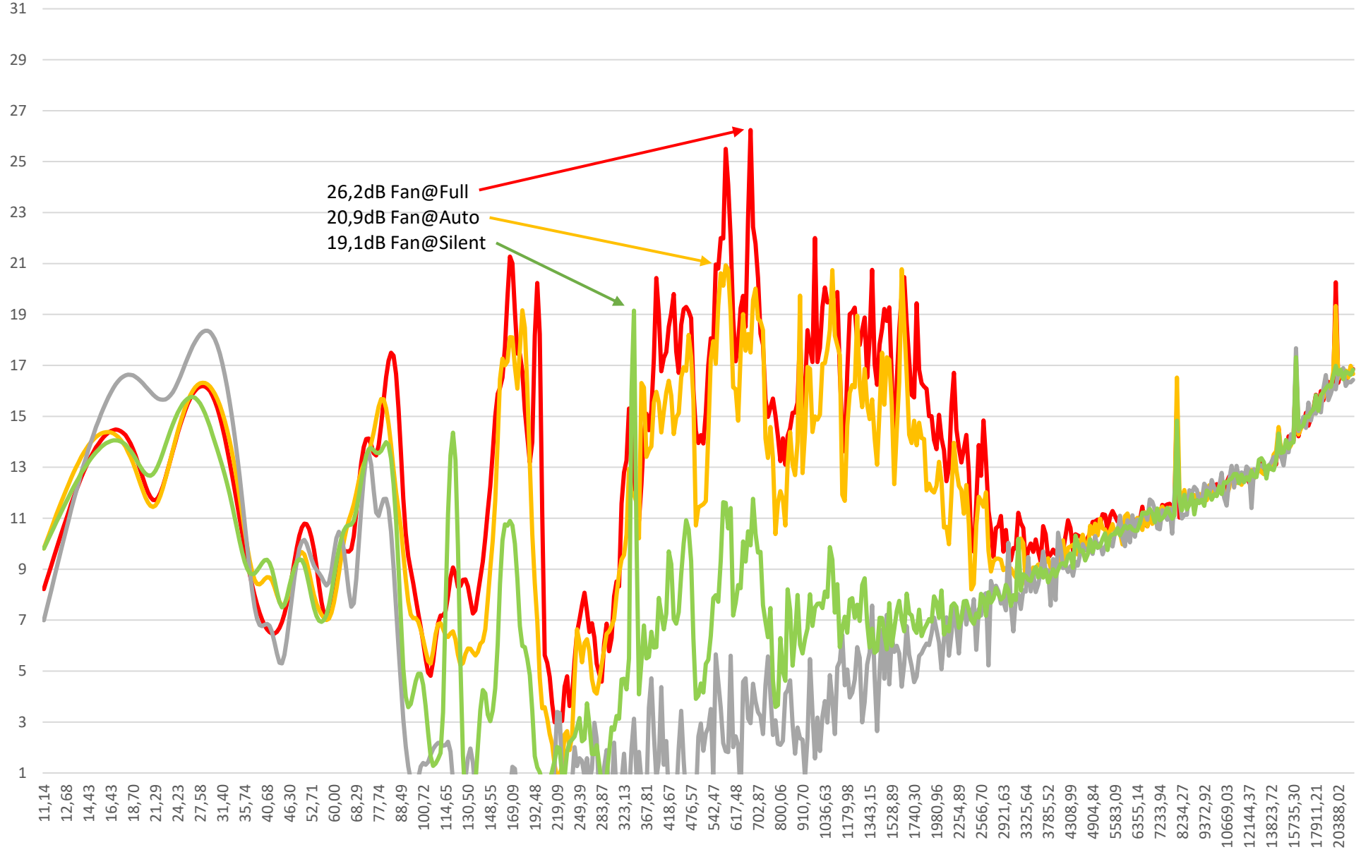
Infinity Signature TCYC-7 Noise Level measurement @ operation temperature 50-55 degrees
