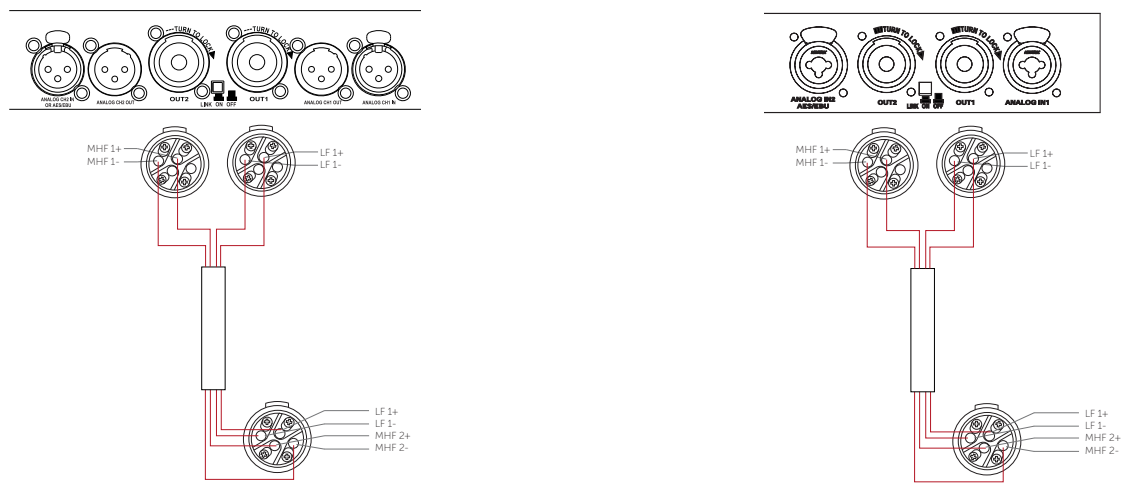
Figure 5.2: Bias V3
