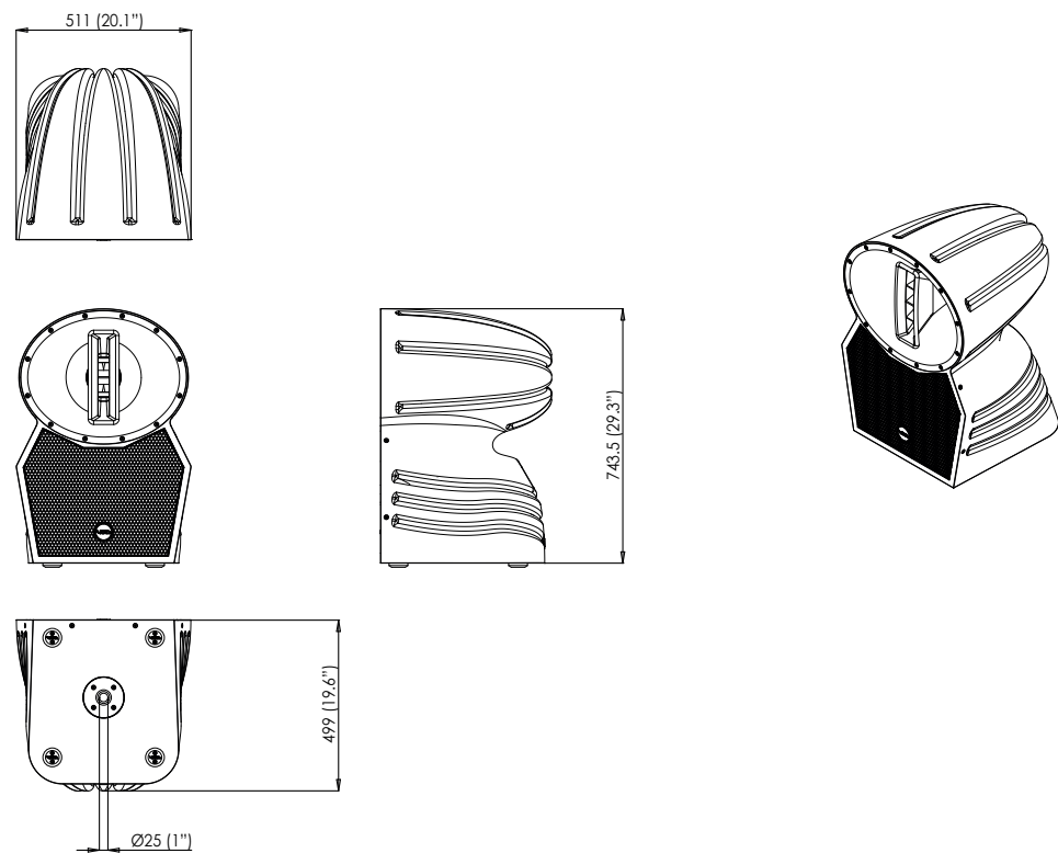
Figure 4.1: Dimensions
