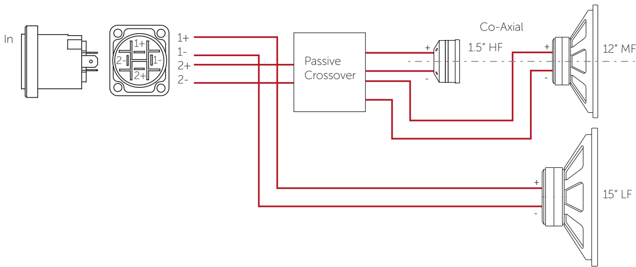
Figure 5.1: Wiring diagram
