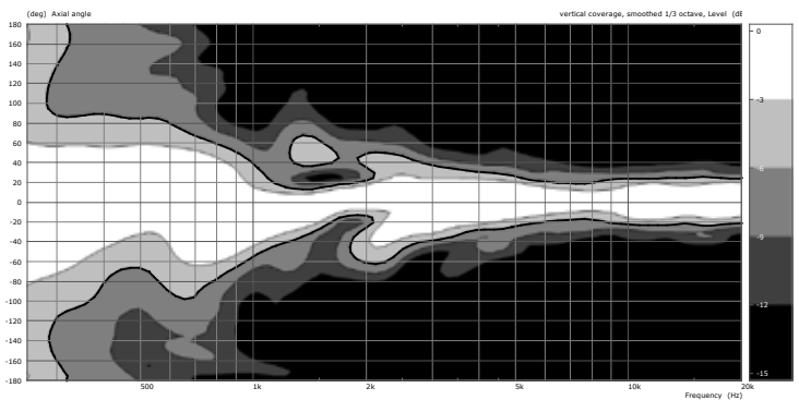
Fig. 4: Vertical coverage
