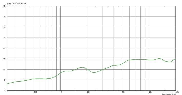
Fig. 5: Directivity index
