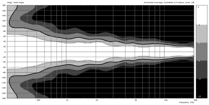
Fig. 2: Horizontal coverage
