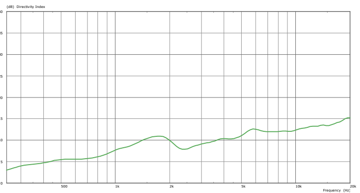
Fig. 5: Directivity index
