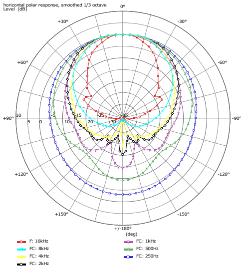
Fig. 1: Horizontal polar pattern
