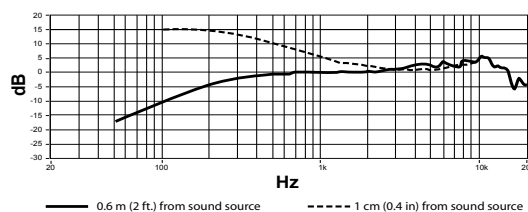
Frequency Response
