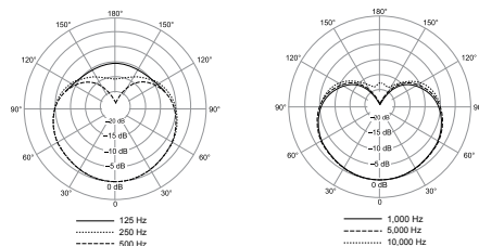
Polar Patterns
