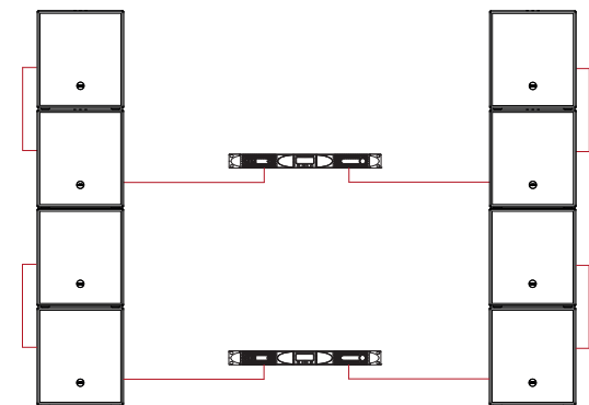
Figure 5.9: 8 x Stasys 118: 4 \Omega per channel / 2 amplifier
