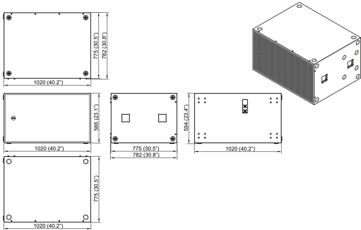
Figure 4.1: Dimensions
