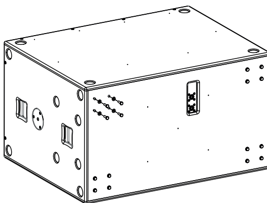
Figure 7.3: Bolt tightening
