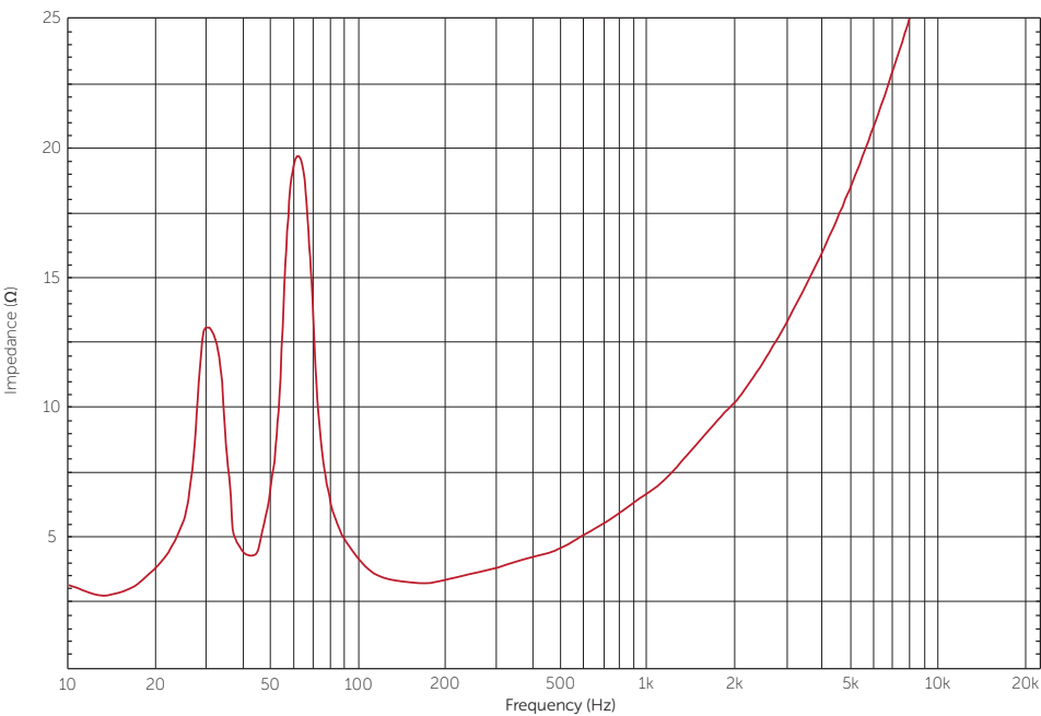
Figure 5.1: Impedance graph
