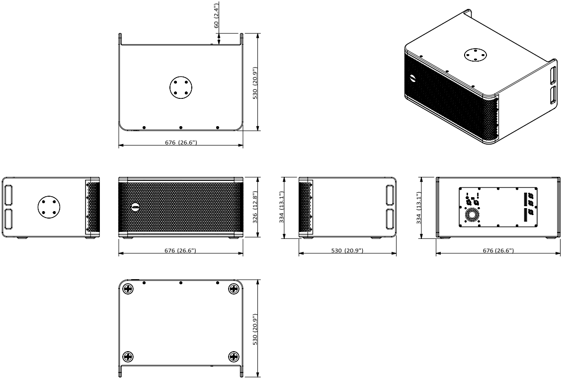
Figure 4.1: Dimensions
