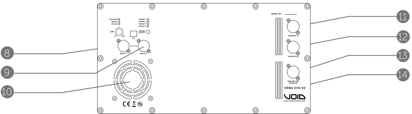
Figure 6.2: Rear panel
