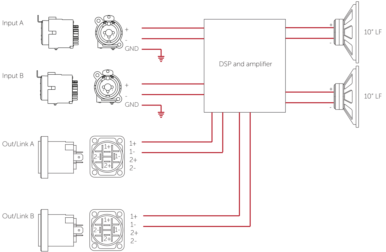
Figure 5.1: Venu 210i V2 wiring diagram
